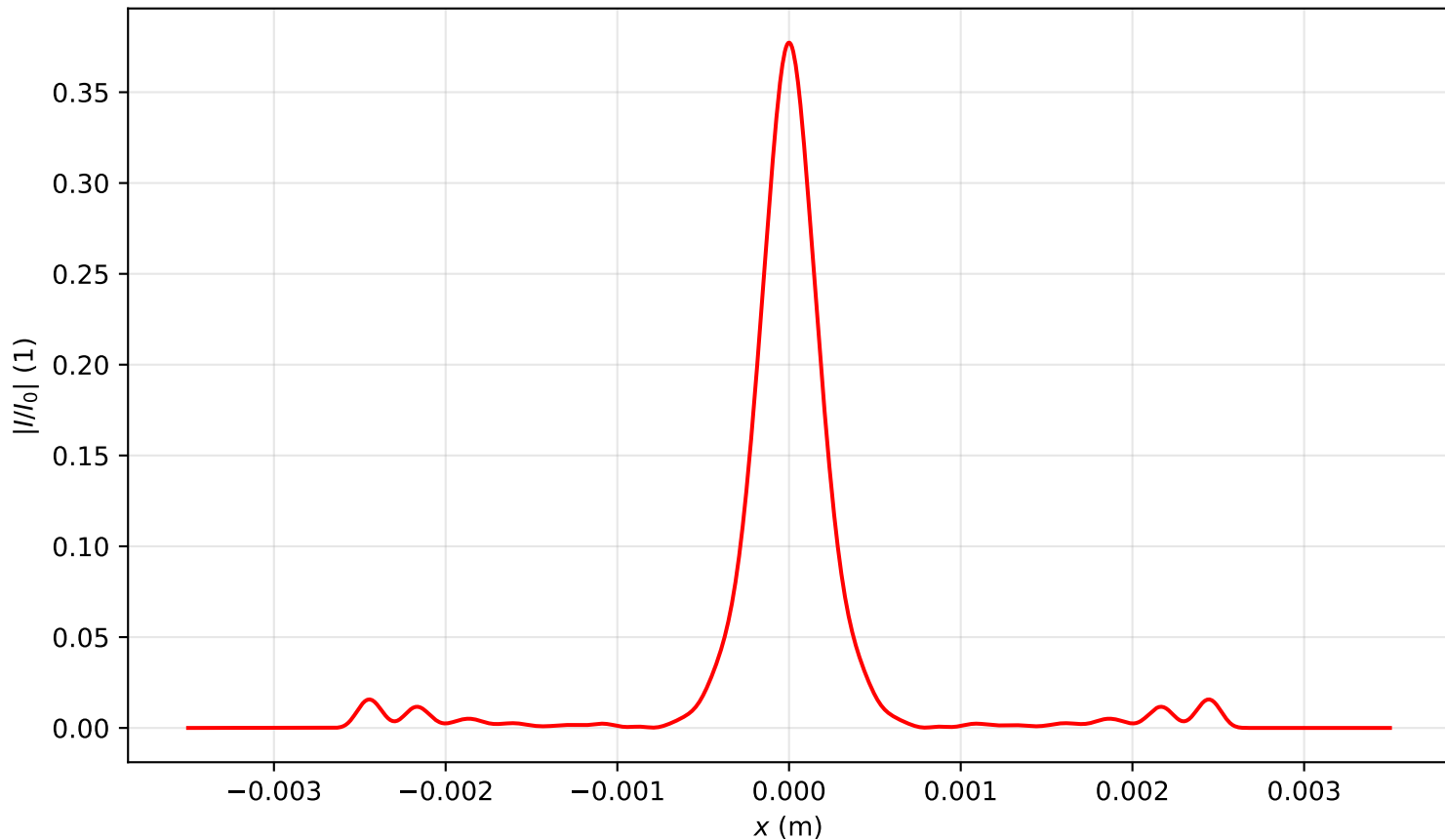
Intensity profile I(x, y = 0, z = 1.911)/I_0 , P_{in}=6.0P_{cr} , artificial time
